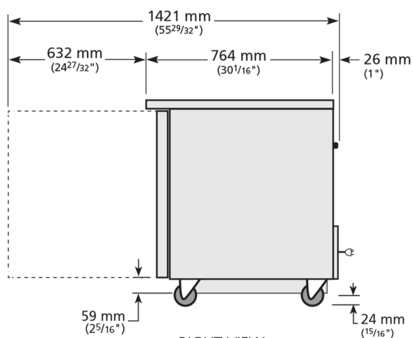
RIGHT VIEW
